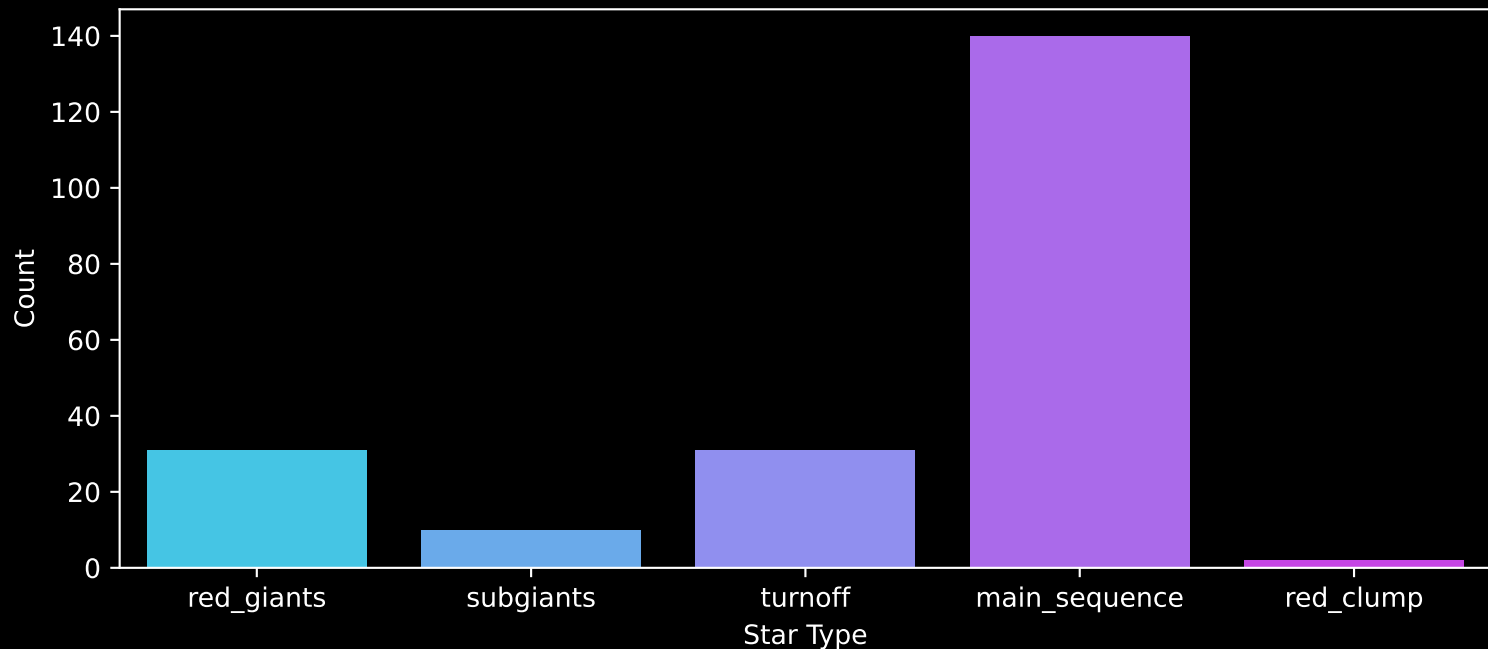
APOGEE DR17 Field: [K2_C14_234+53] Count plot of Star Type
