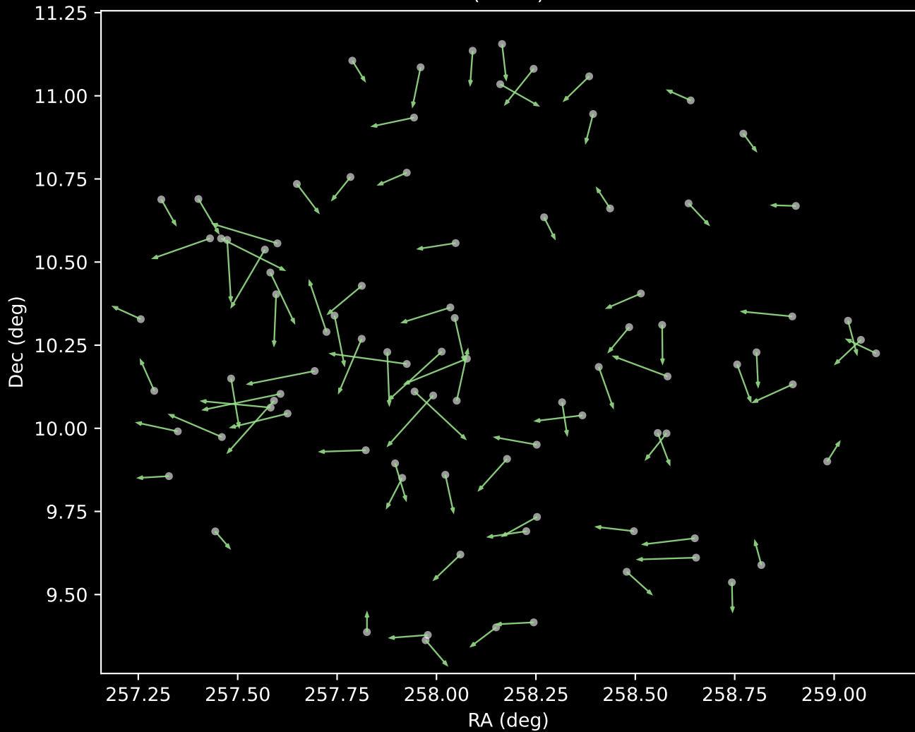
APOGEE DR17 Cluster 5 Proper Motion Vectors (n=90)
