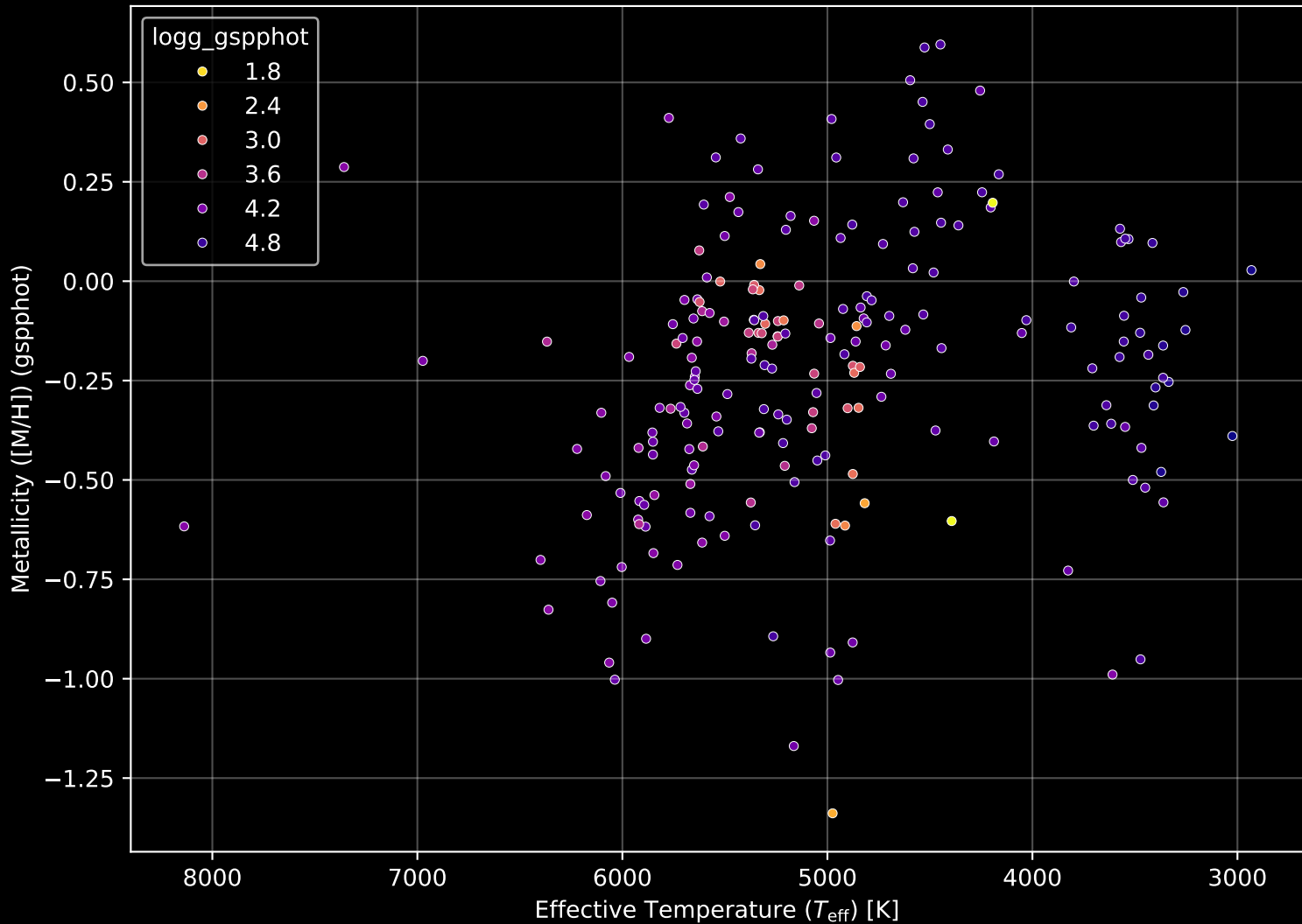
APOGEE DR17 Field: [K2_C14_234+53] Stellar Population Parameters (n= 214)
