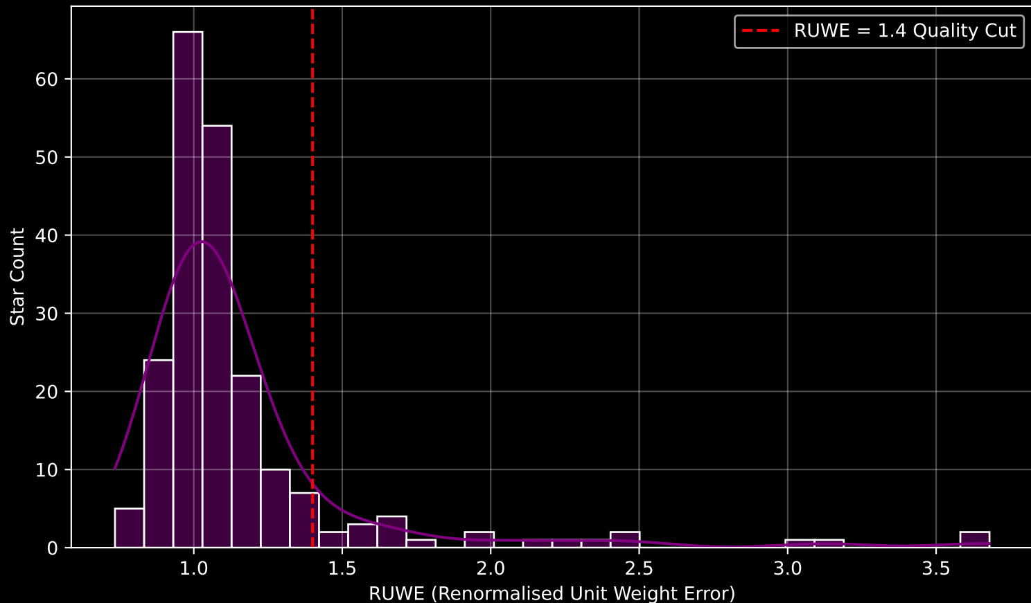
GAPOGEE DR17 Field [K2_C14_234+53] RUWE Distribution (n= 209)
