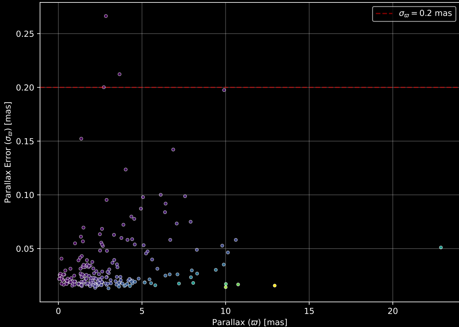
APOGEE DR17 Field: [K2_C14_234+53] Parallax Quality (n= 214)
