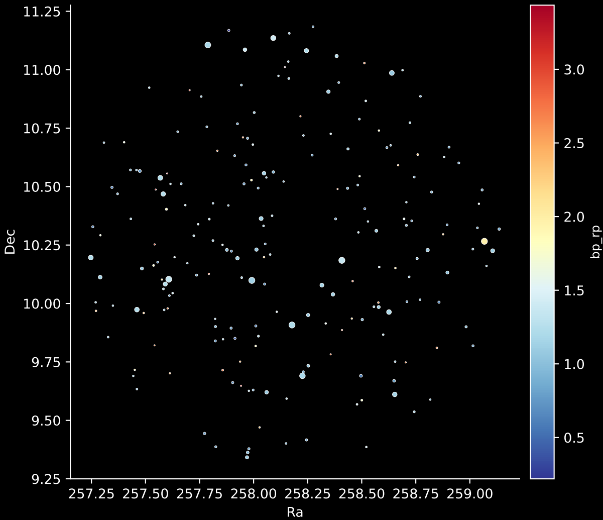
APOGEE DR17 Field: [K2_C14_234+53] Stars: 214
