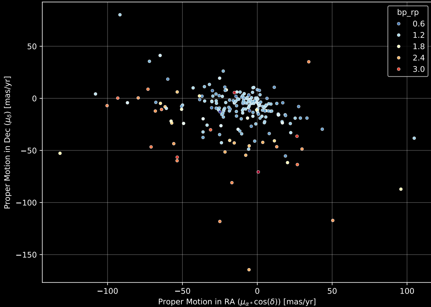
APOGEE DR17 Field: [K2_C14_234+53] Proper Motion Diagram (n= 214)
