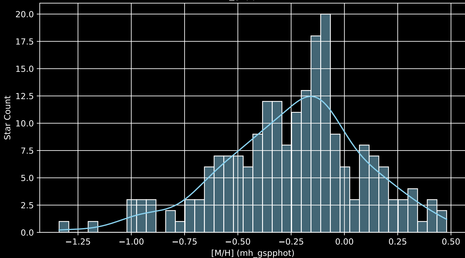
APOGEE DR17 Field: [K2_C14_234+53 [M/H] (mh_gspphot) (n= 211)
